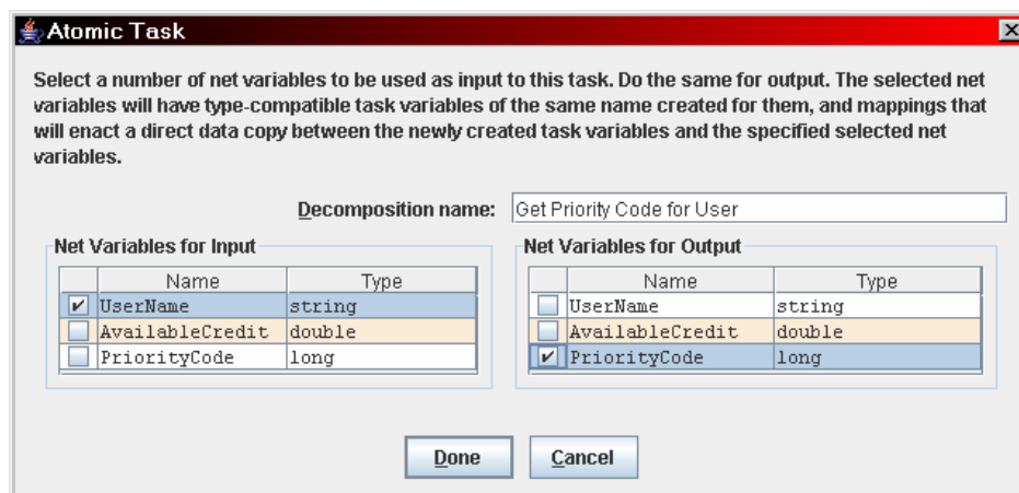
Fig. 42: An example of the direct data transfer dialog
