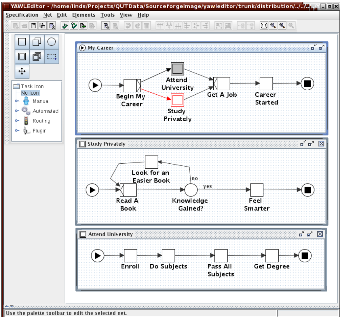
Fig. 35: The complete scenario specification
