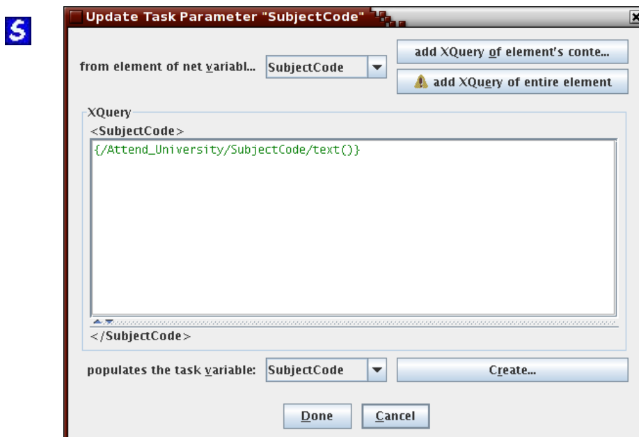
Fig. 32: Passing a net's SubjectCode value to a Task
