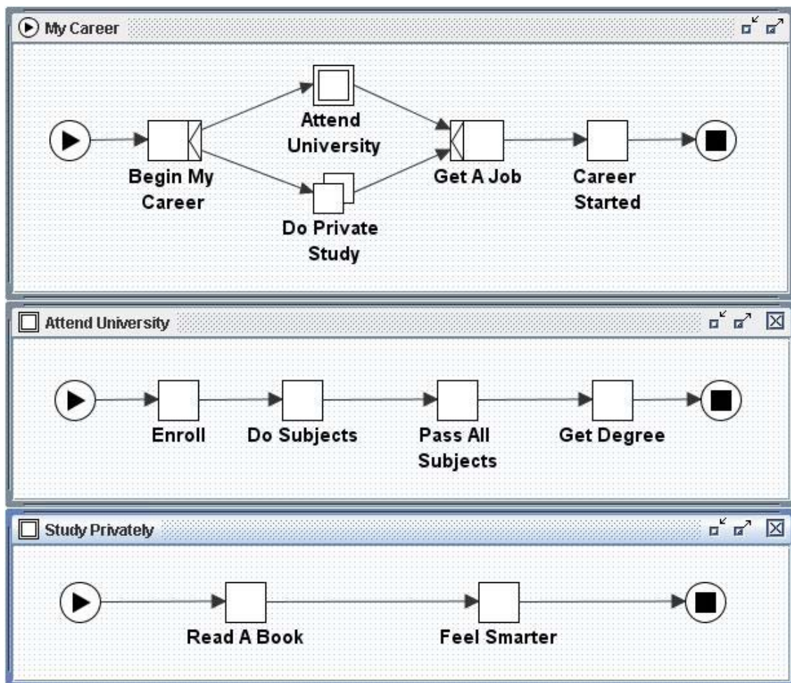
Fig. 12. "Privately Study" Multiple Composite Task and its Net
