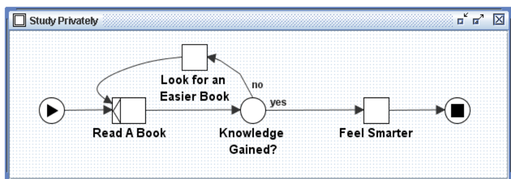
Fig. 17: Adding "knees" to a Flow Relation
