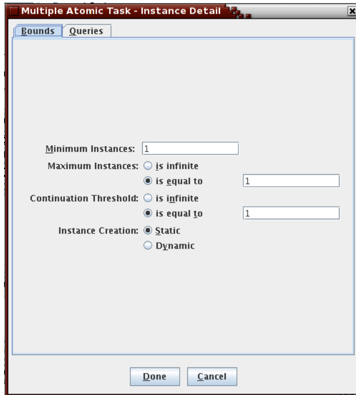
Fig. 11: Instance Bounds on Multiple Instance Tasks
