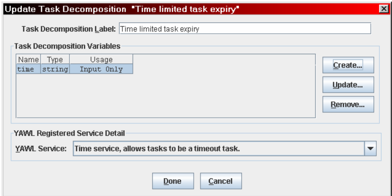
Fig. 46 - Assigning a registered YAWL service from a running engine
