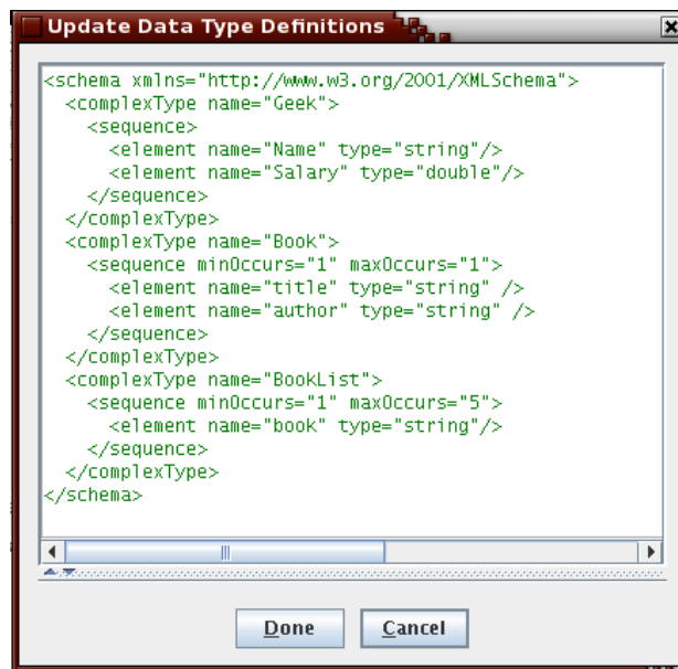
Fig. 21: Adding the "Geek" complex data type
