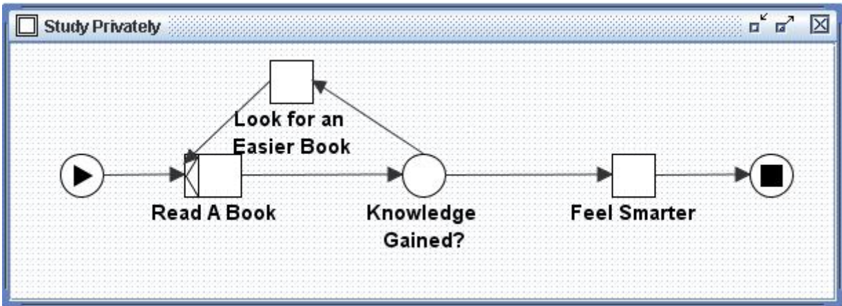
Fig. 13. Condition Loop for “Study Privately” Net
