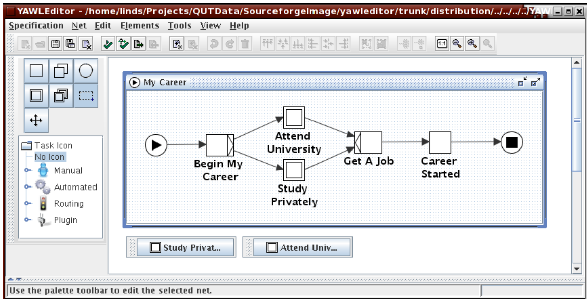
Fig. 15: Making the "Study Privately" task an atomic composite
