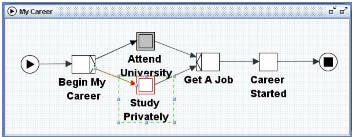
Fig. 20. Adding elements to a Cancellation Set
