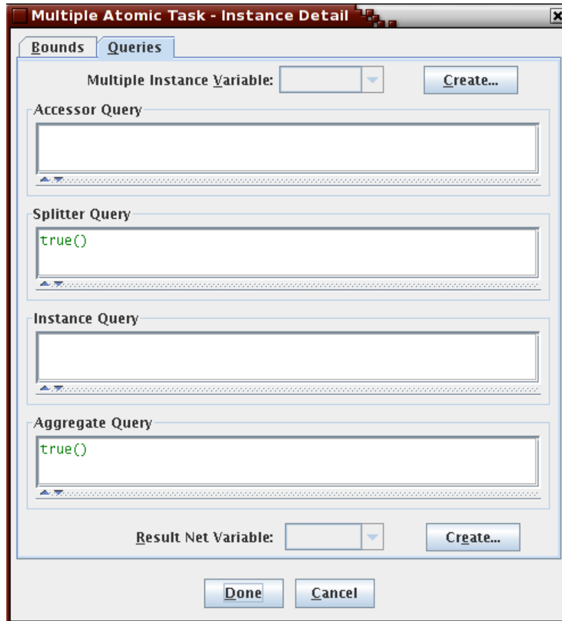
Fig. 37: Data manipulation for Multiple Instance Tasks
