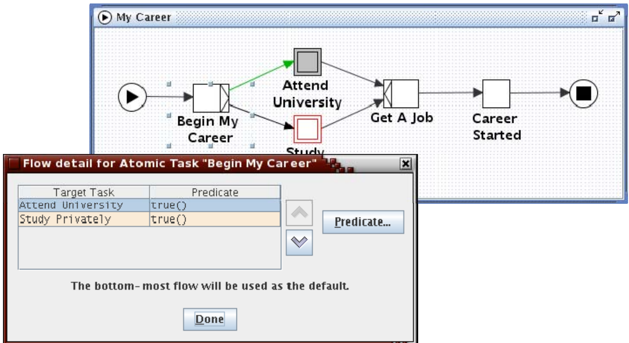
Fig. 34: Updating the Flow Detail
