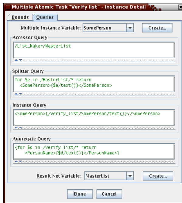
Fig. 44: Example multiple instance queries
