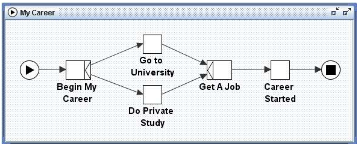
Fig. 8: XOR Split and Join
