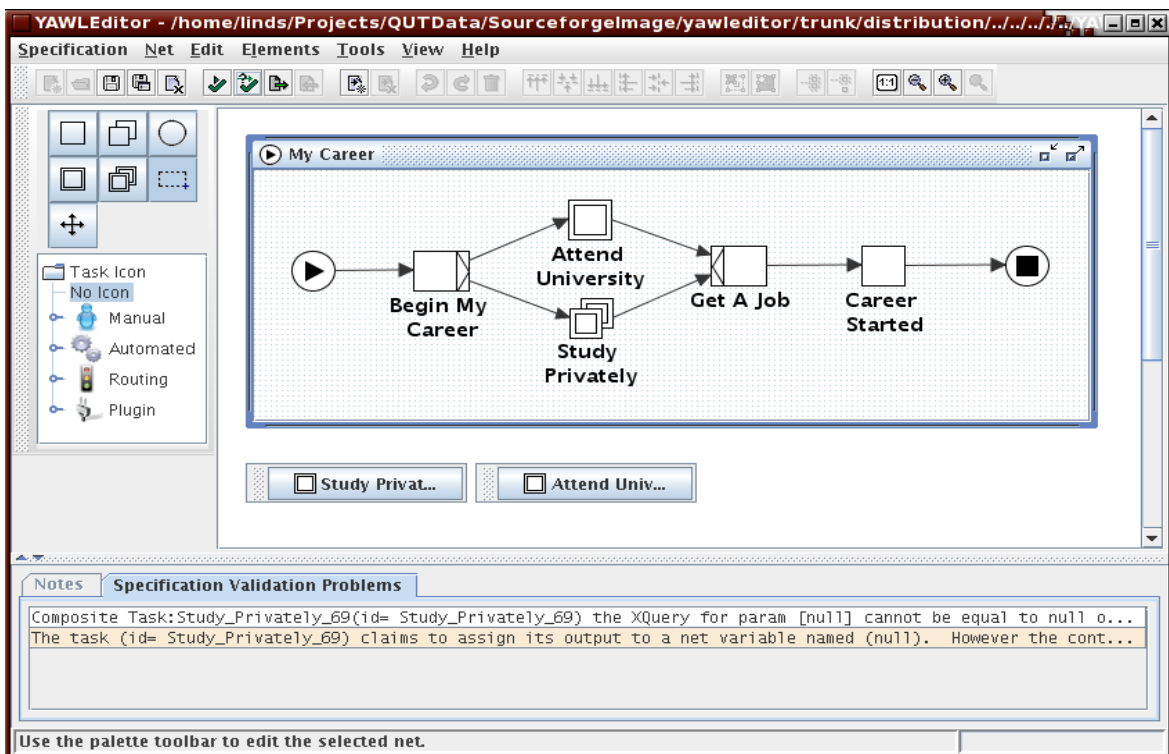
Fig. 14: Validation with unfinished Multiple-Instance Tasks
