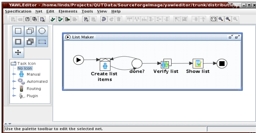
Fig. 43: A simple specification showcasing multiple instance tasks
