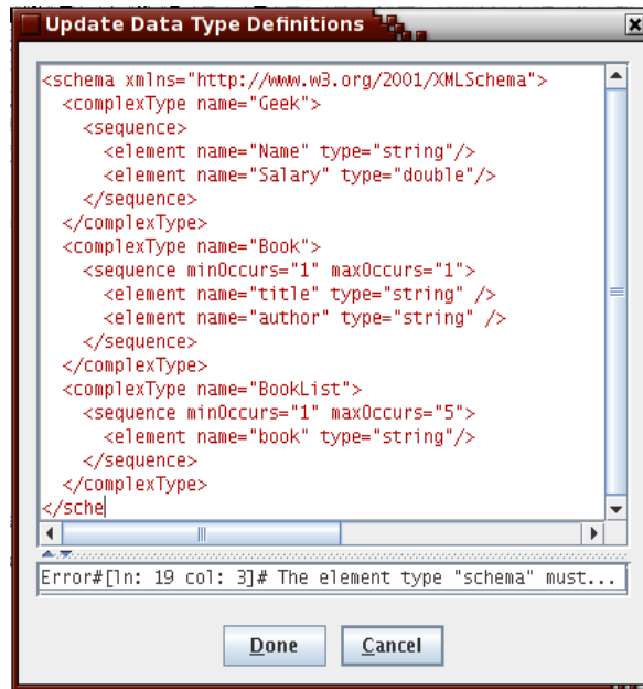
Fig. 22: When the "Geek" complex data type scheme is invalid
