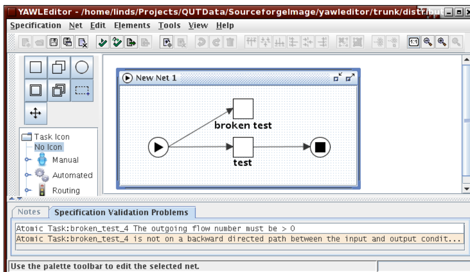
Fig. 39: An invalid specification
