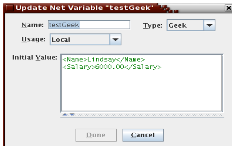
Fig. 23: A "Geek" net variable with initial value
