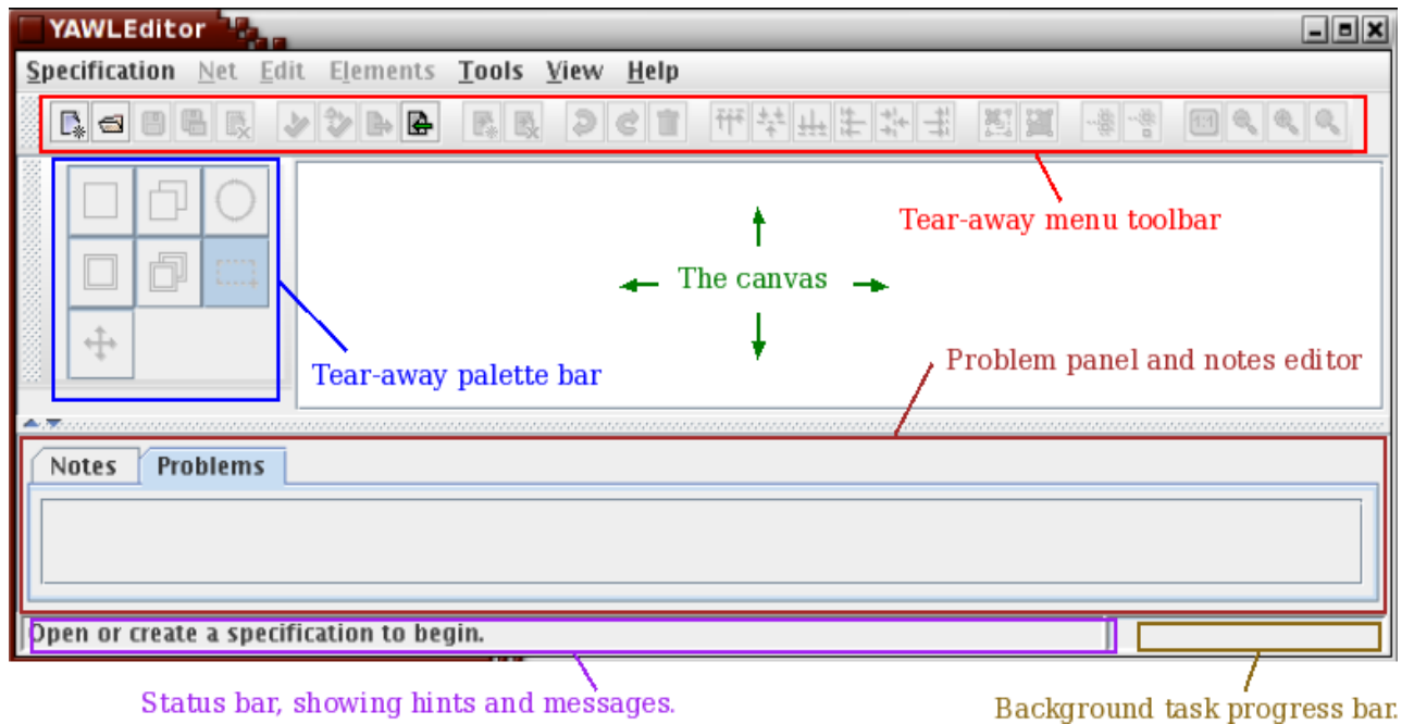
Fig. 2. The YAWLEditor Workspace
