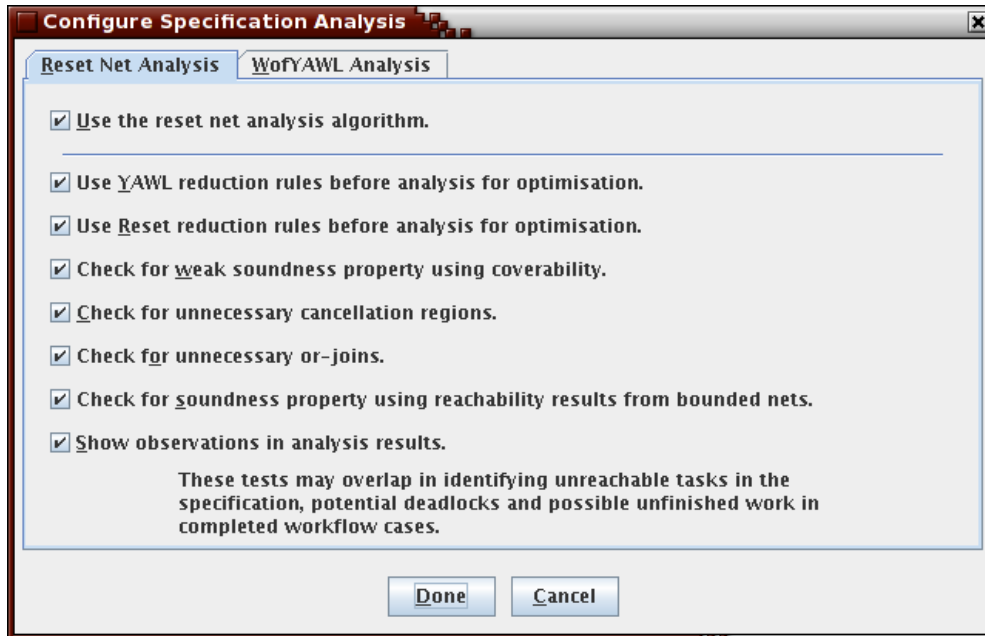
Fig. 40: Specification analysis configuration
