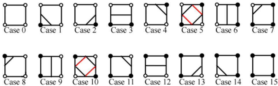
Figure 6: The 16 marching square cases
