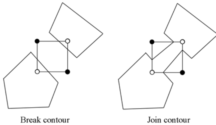
Figure 7: Two ambiguous cases in the marching squares algorithm
